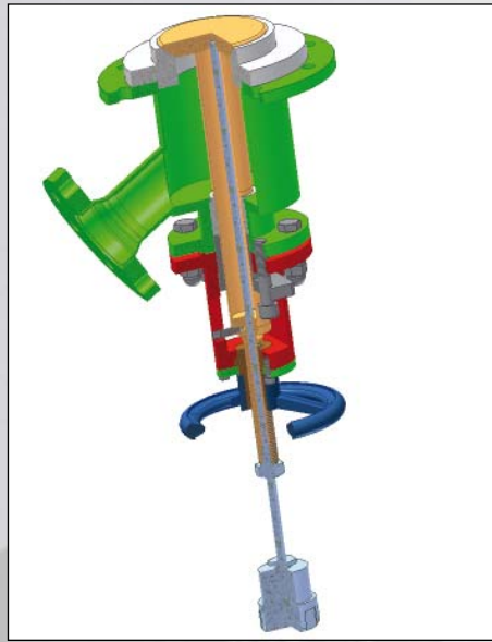
A draining valve
