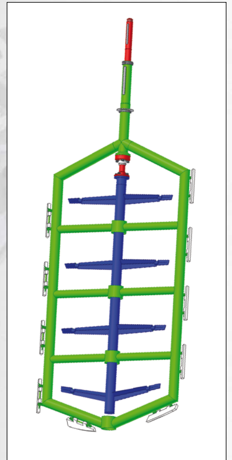
A gate agitator with scrapers and a counter-rotating paddle agitator
